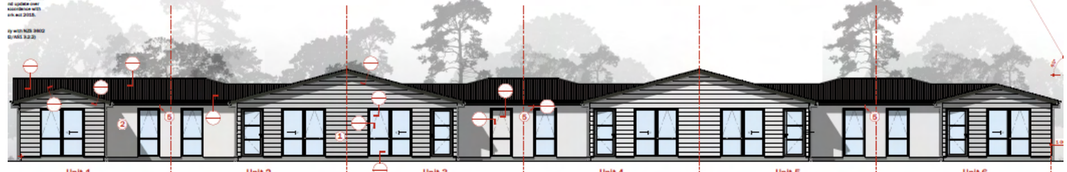
Elevations - Exterior - Elevation B 1 mm = 100 mm
