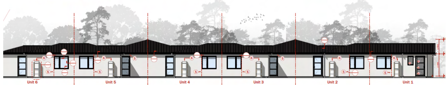
Elevations - Exterior - Elevation D 1 mm = 100 mm
